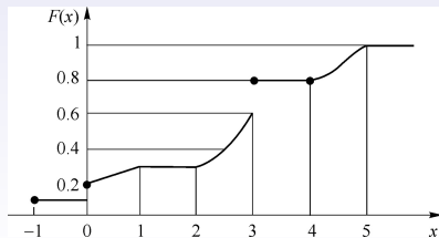
Figure: d.f. of Example 1
